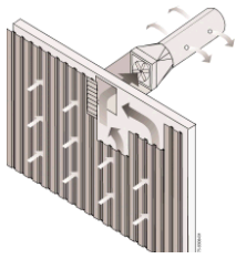
Transpired collector components (NREL)
