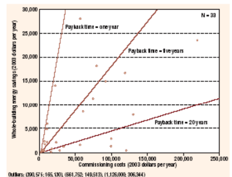
Figure 2. Cost, savings, and payback time of new construction building commissioning
